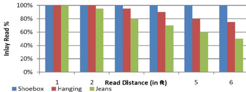
Fig 6: Configuration Variation Effects: Inlay read performance for varying arrangements
