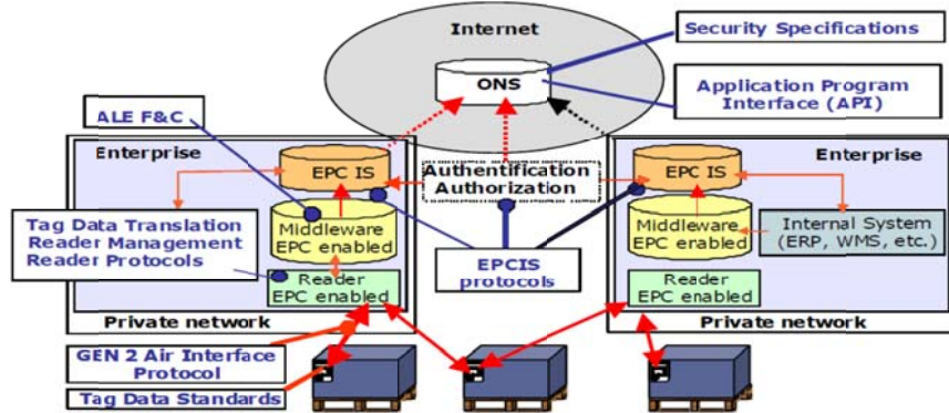
Fig 1: EPCglobal Network Standards (Source: GS1 Germany/EPCglobal)
