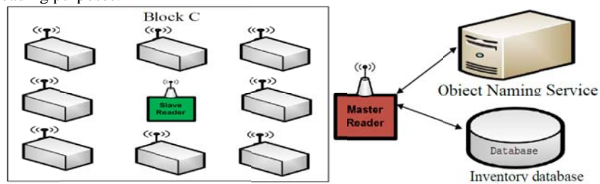
Fig 3 (a) Block Structure (b) Communication of Master reader with ONS and Inventory database We have made following assumption in proposing our system architecture:
