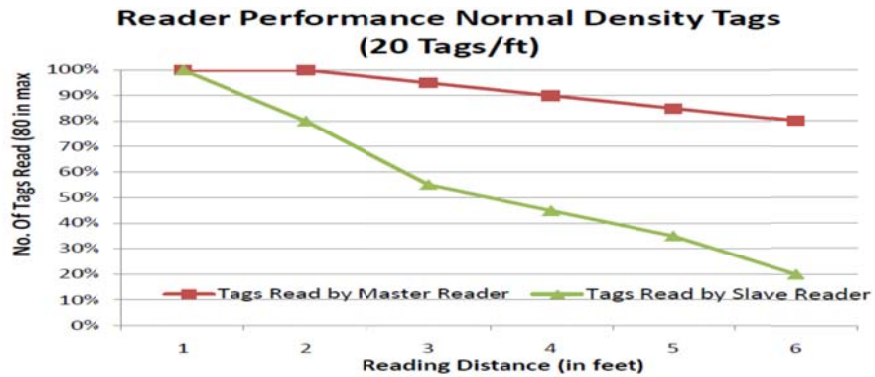
Fig 7: Reading Performance comparison of master and Slave Tag Readers
